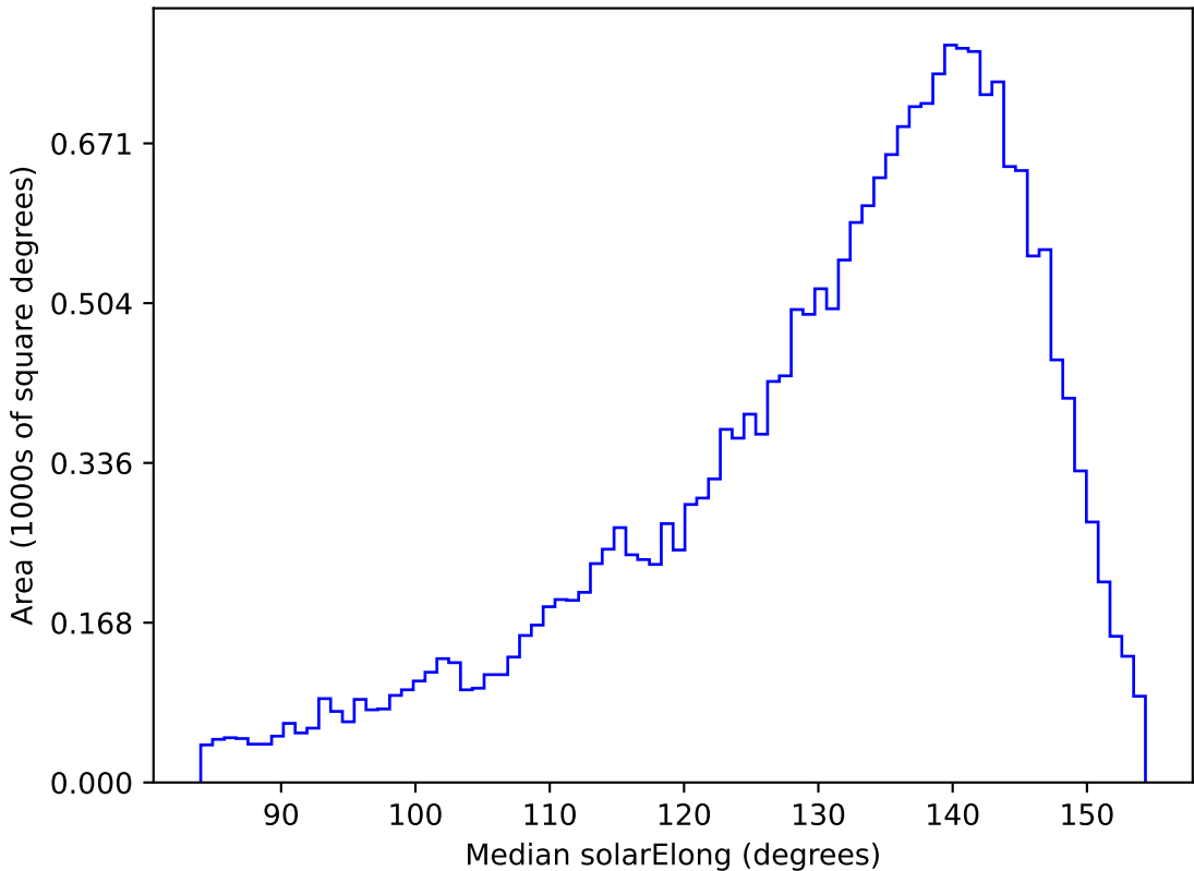
too_ignore_5_1v3.4_10yrs All sky u band: Median solarElong
