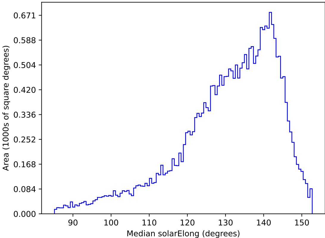
too_ignore_5_1v3.4_10yrs All sky r band: Median solarElong
