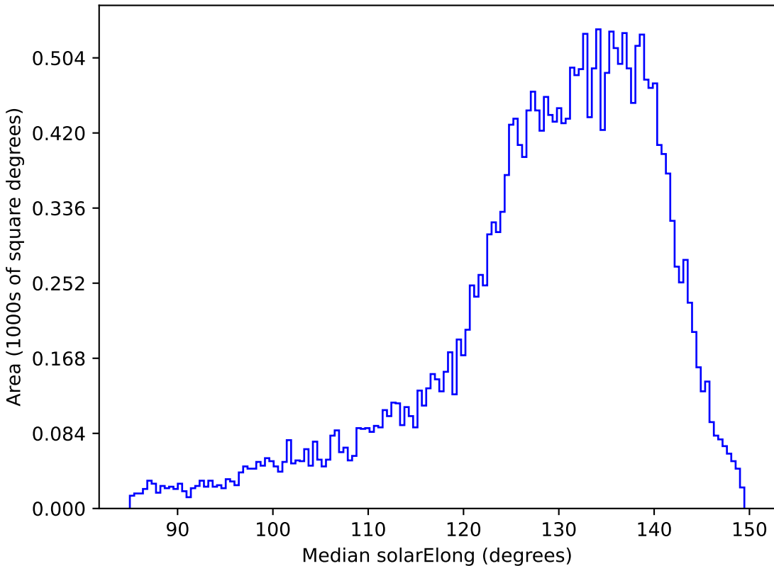
too_ignore_5_1v3.4_10yrs All sky i band: Median solarElong
