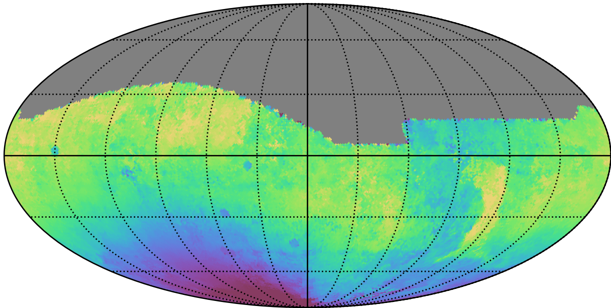
too_ignore_5_1v3.4_10yrs All sky g band: Median solarElong
