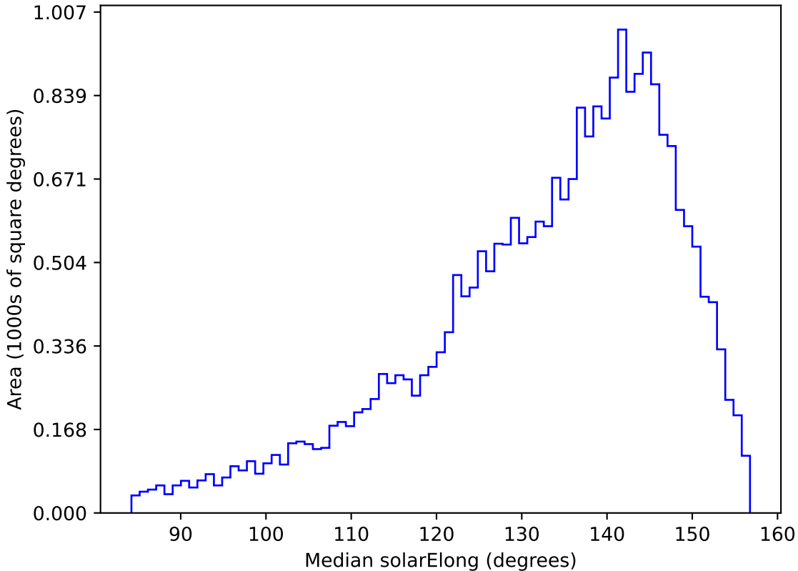
too_ignore_5_1v3.4_10yrs All sky g band: Median solarElong
