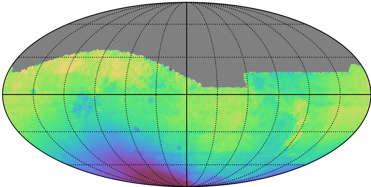
too_ignore_5_1v3.4_10yrs All sky all bands: Median solarElong
