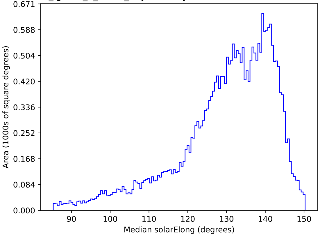
too_ignore_5_1v3.4_10yrs All sky all bands: Median solarElong
