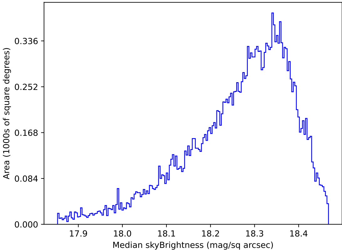
too_ignore_5_1v3.4_10yrs Yr 1 y band: Median skyBrightness
