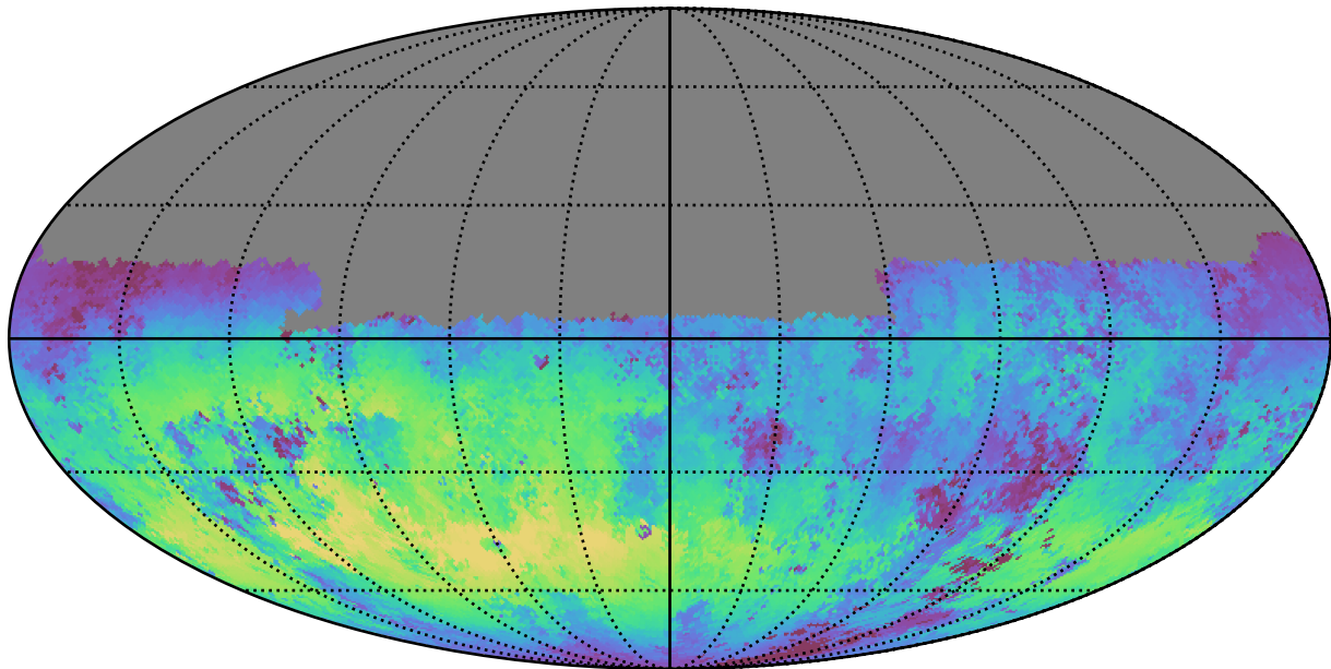
too_ignore_5_1v3.4_10yrs Yr 1 u band: Median skyBrightness
