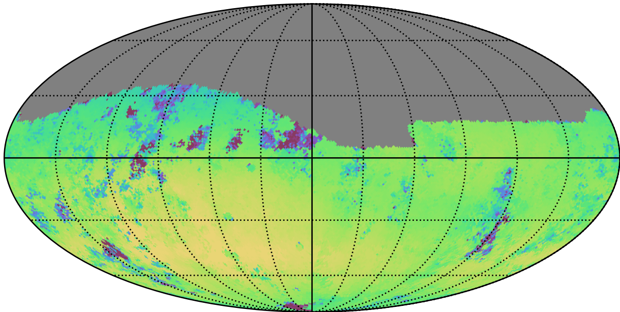
too_ignore_5_1v3.4_10yrs Yr 1 r band: Median skyBrightness
