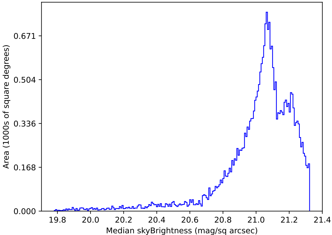
too_ignore_5_1v3.4_10yrs Yr 1 r band: Median skyBrightness
