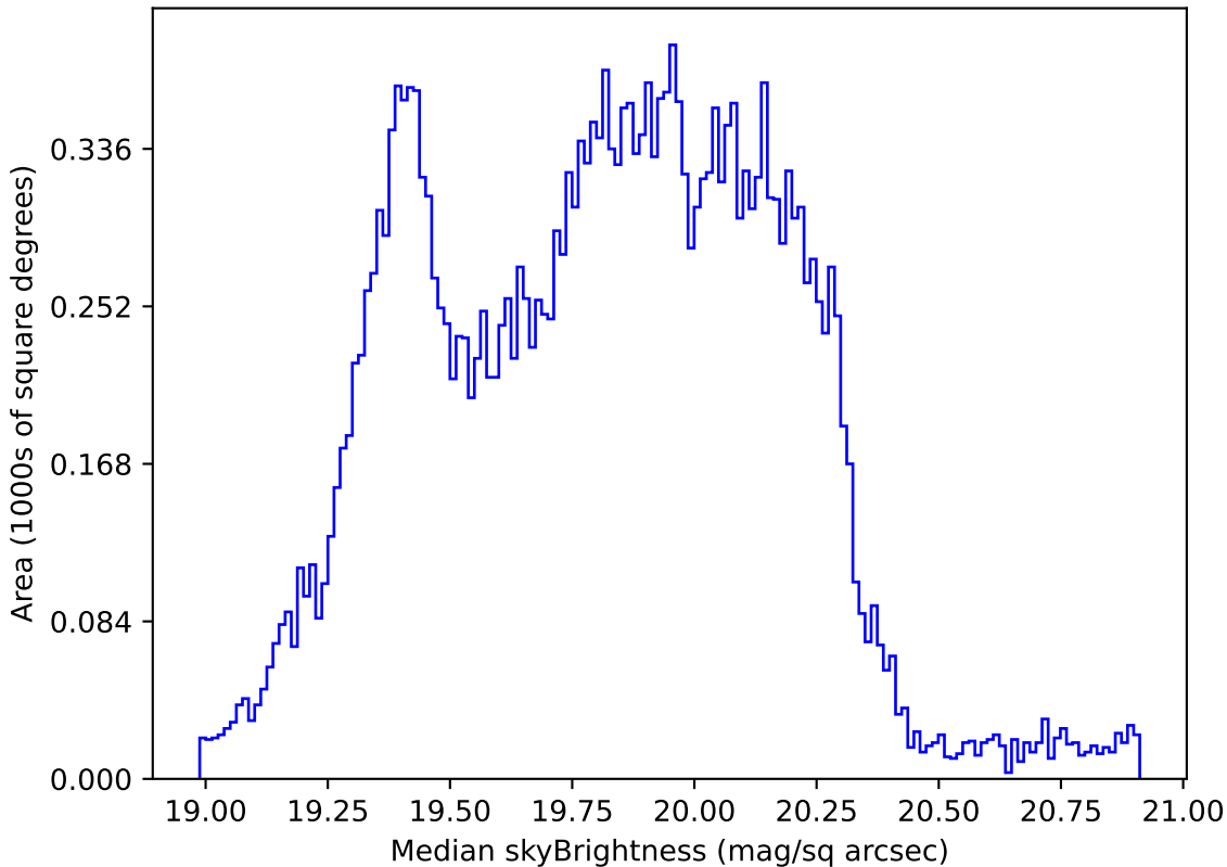
too_ignore_5_1v3.4_10yrs Yr 1 all bands: Median skyBrightness
