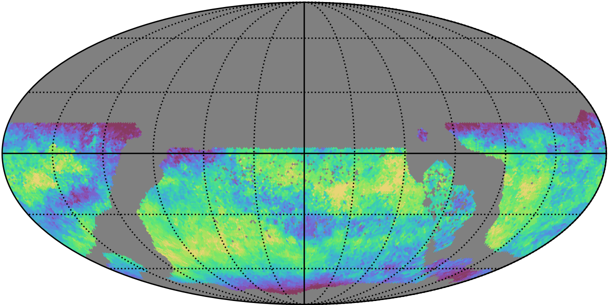
too_ignore_5_1v3.4_10yrs WFD z band: Median skyBrightness
