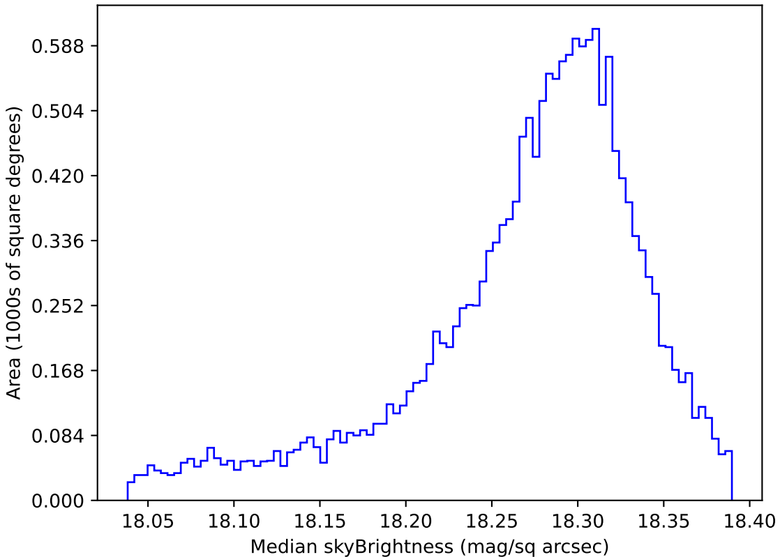
too_ignore_5_1v3.4_10yrs WFD y band: Median skyBrightness
