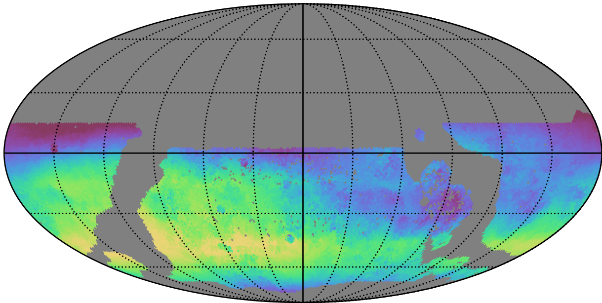
too_ignore_5_1v3.4_10yrs WFD u band: Median skyBrightness
