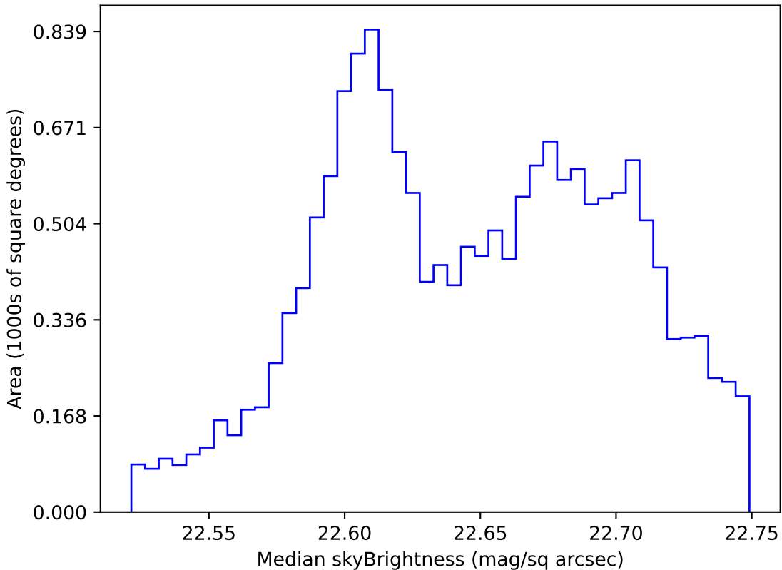
too_ignore_5_1v3.4_10yrs WFD u band: Median skyBrightness
