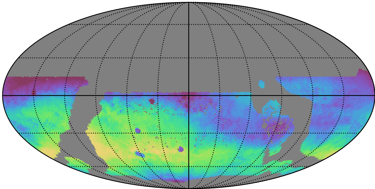
too_ignore_5_1v3.4_10yrs WFD r band: Median skyBrightness
