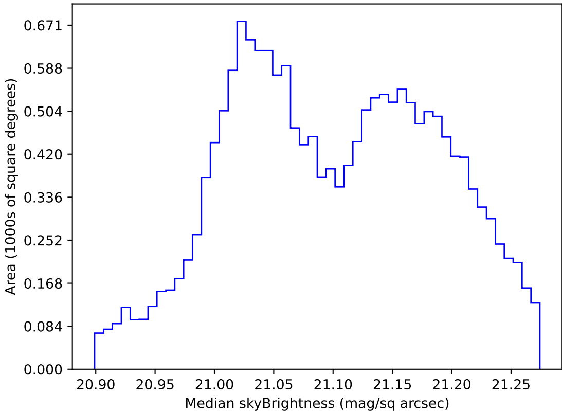
too_ignore_5_1v3.4_10yrs WFD r band: Median skyBrightness
