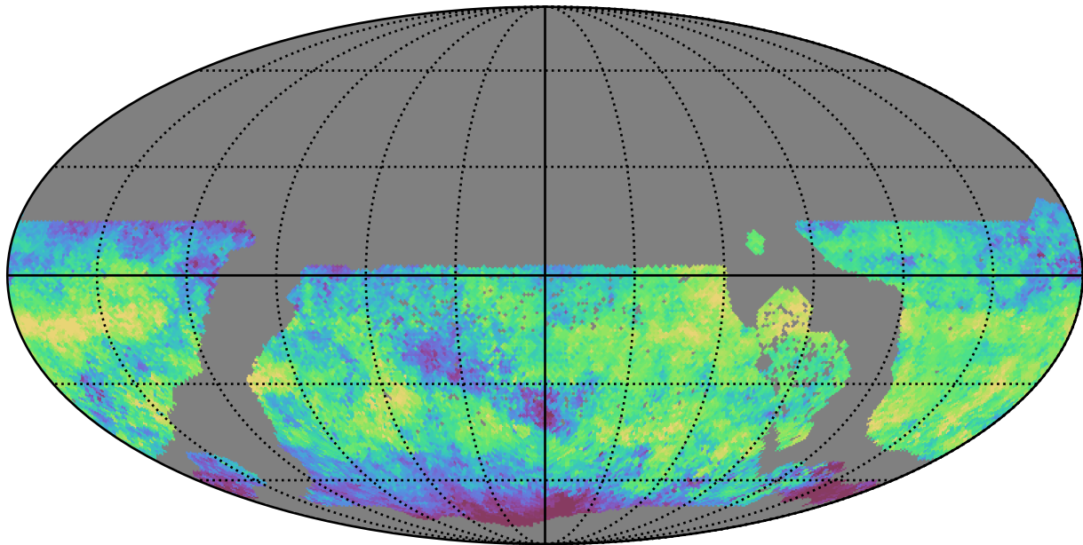
too_ignore_5_1v3.4_10yrs WFD i band: Median skyBrightness
