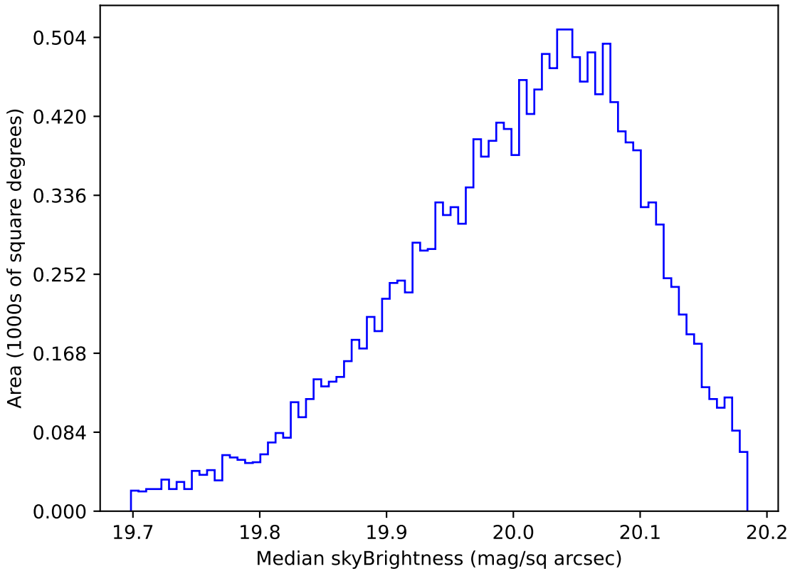
too_ignore_5_1v3.4_10yrs WFD i band: Median skyBrightness
