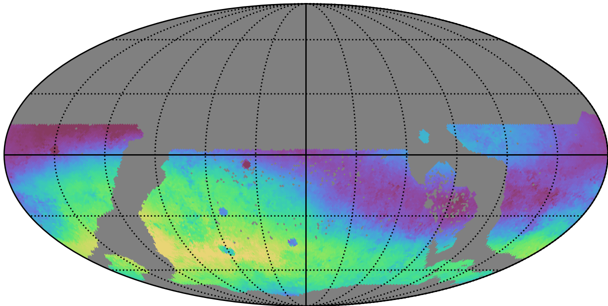
too_ignore_5_1v3.4_10yrs WFD g band: Median skyBrightness
