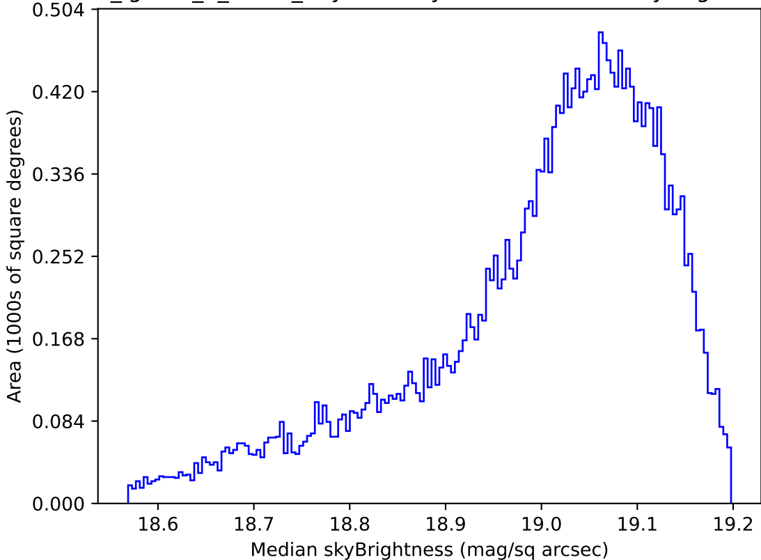
too_ignore_5_1v3.4_10yrs All sky z band: Median skyBrightness
