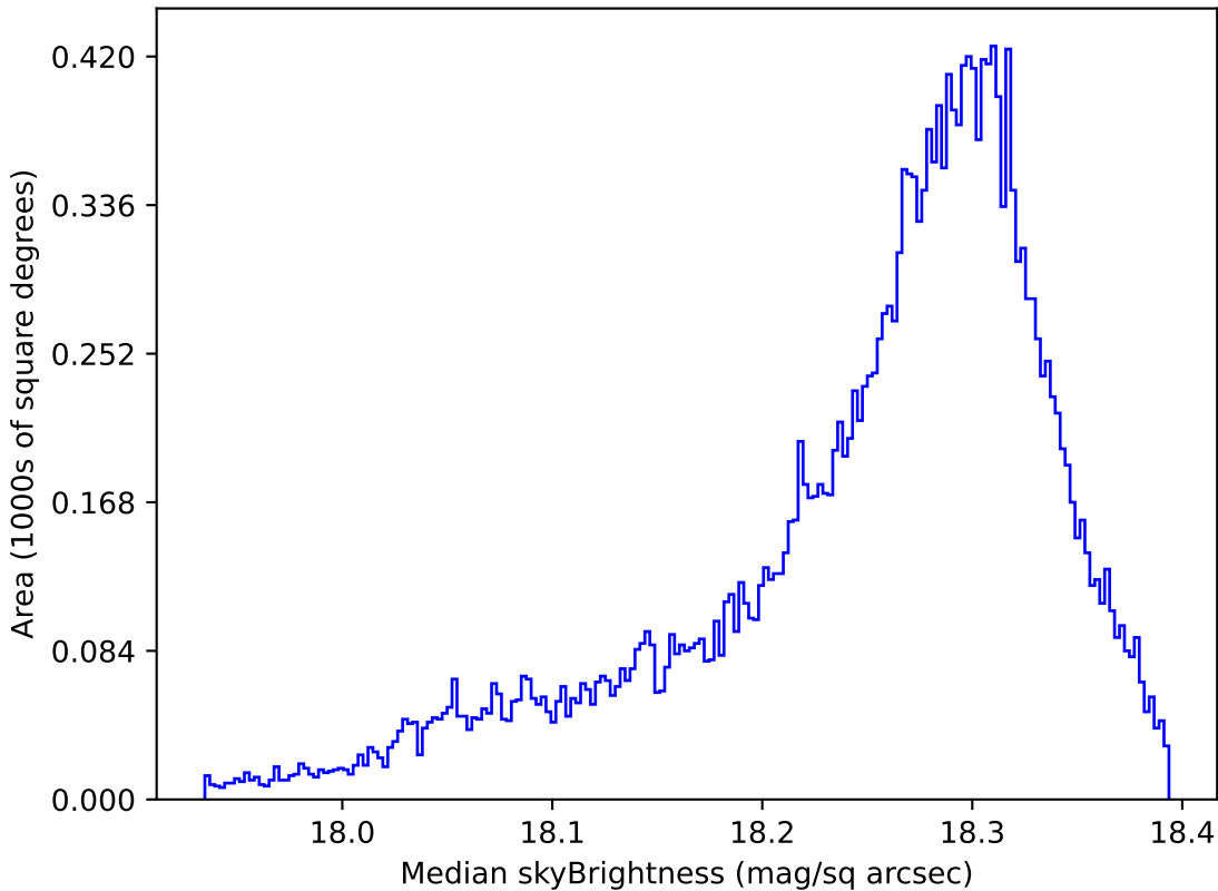
too_ignore_5_1v3.4_10yrs All sky y band: Median skyBrightness
