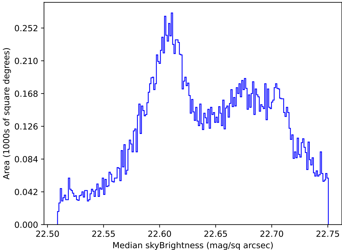
too_ignore_5_1v3.4_10yrs All sky u band: Median skyBrightness
