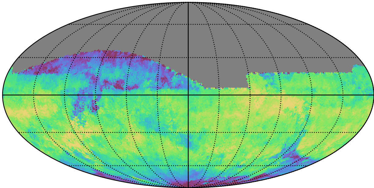
too_ignore_5_1v3.4_10yrs All sky i band: Median skyBrightness
