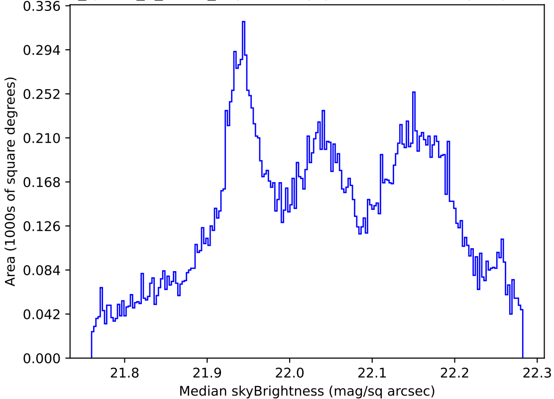
too_ignore_5_1v3.4_10yrs All sky g band: Median skyBrightness
