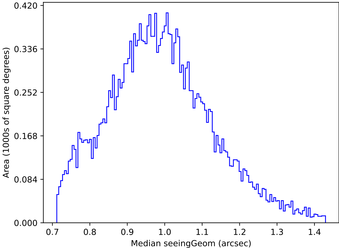
too_ignore_5_1v3.4_10yrs Yr 1 u band: Median seeingGeom
