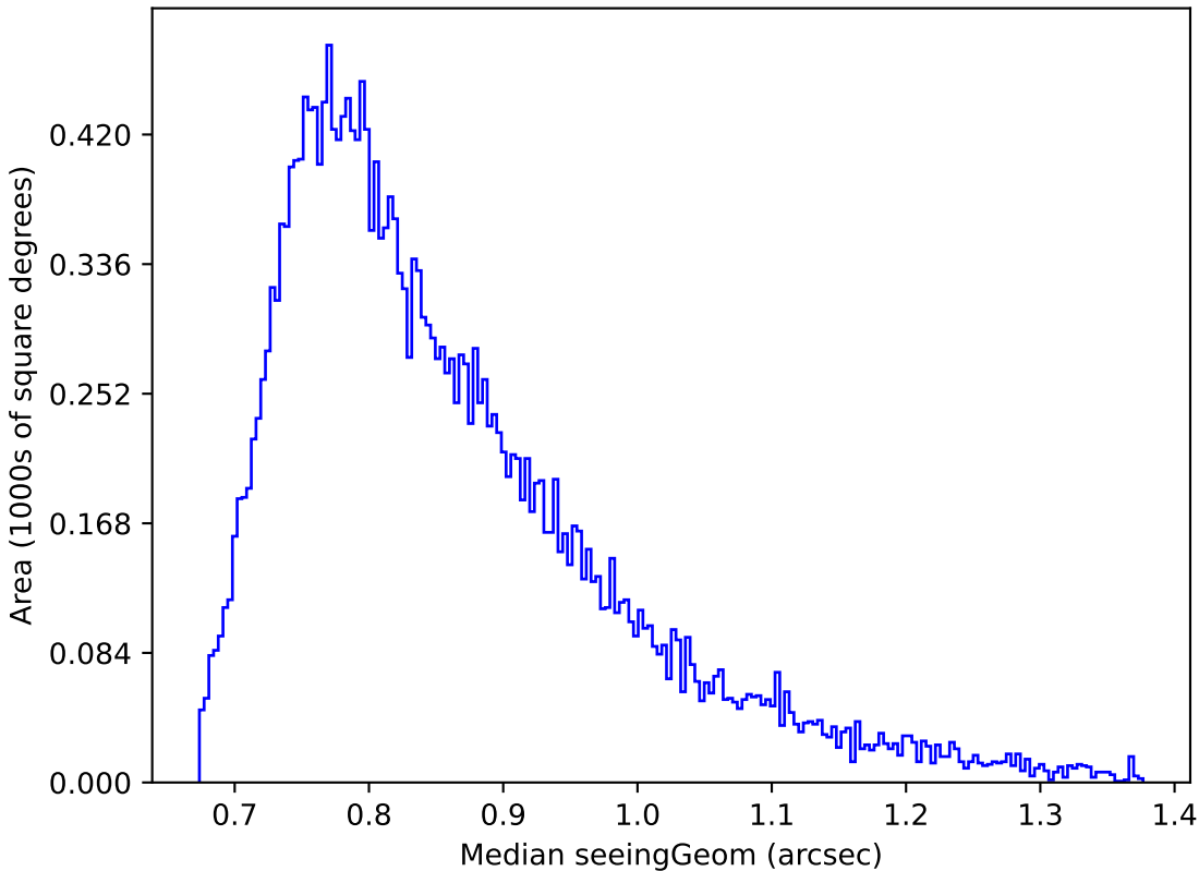
too_ignore_5_1v3.4_10yrs Yr 1 r band: Median seeingGeom
