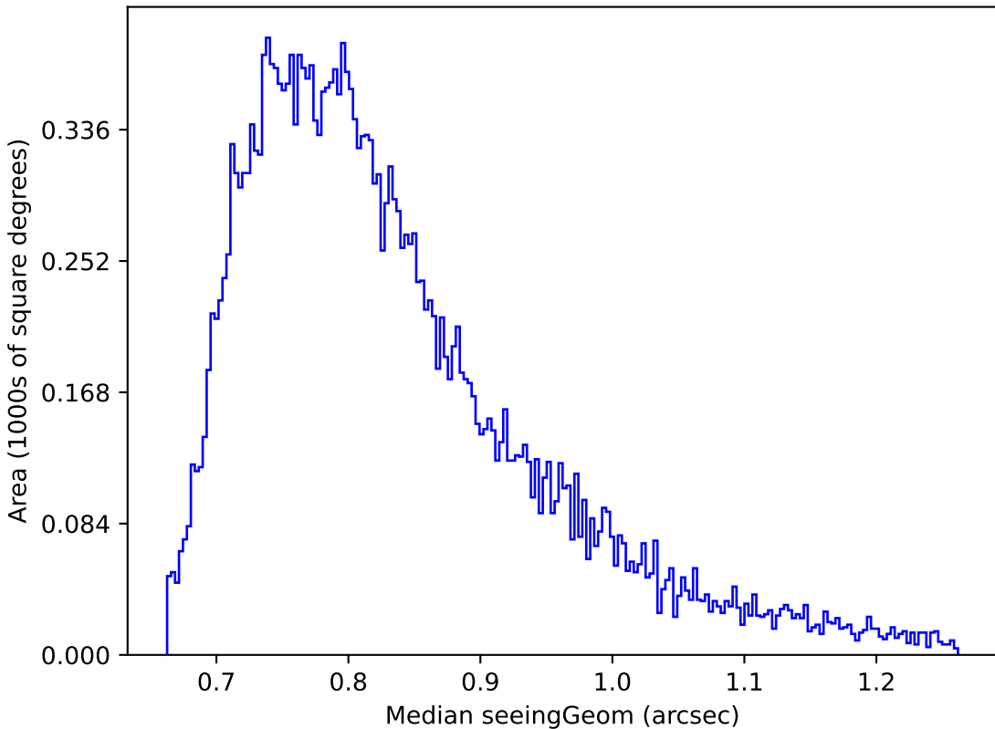
too_ignore_5_1v3.4_10yrs Yr 1 i band: Median seeingGeom
