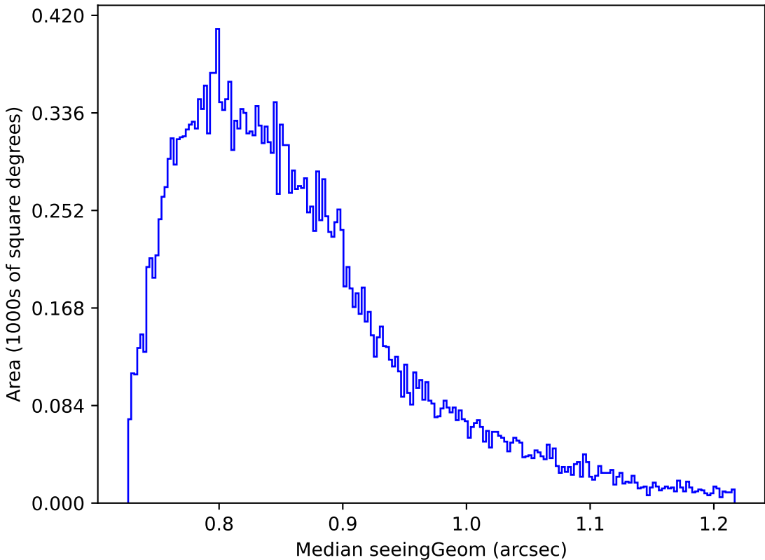
too_ignore_5_1v3.4_10yrs Yr 1 all bands: Median seeingGeom
