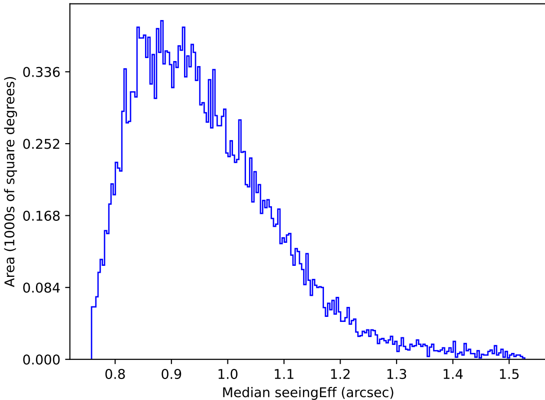
too_ignore_5_1v3.4_10yrs Yr 1 z band: Median seeingEff
