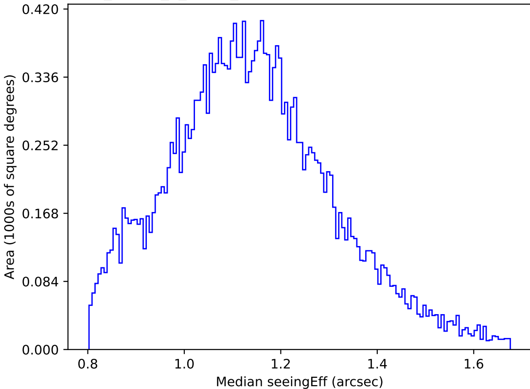
too_ignore_5_1v3.4_10yrs Yr 1 u band: Median seeingEff
