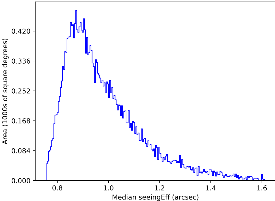
too_ignore_5_1v3.4_10yrs Yr 1 r band: Median seeingEff
