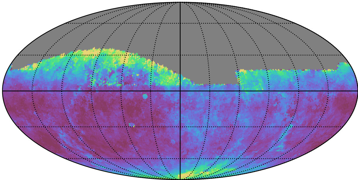
too_ignore_5_1v3.4_10yrs Yr 1 all bands: Median seeingEff
