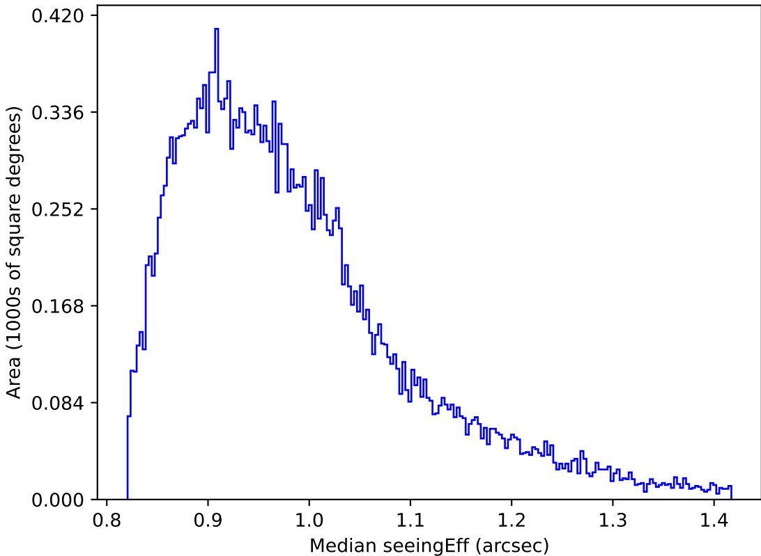
too_ignore_5_1v3.4_10yrs Yr 1 all bands: Median seeingEff
