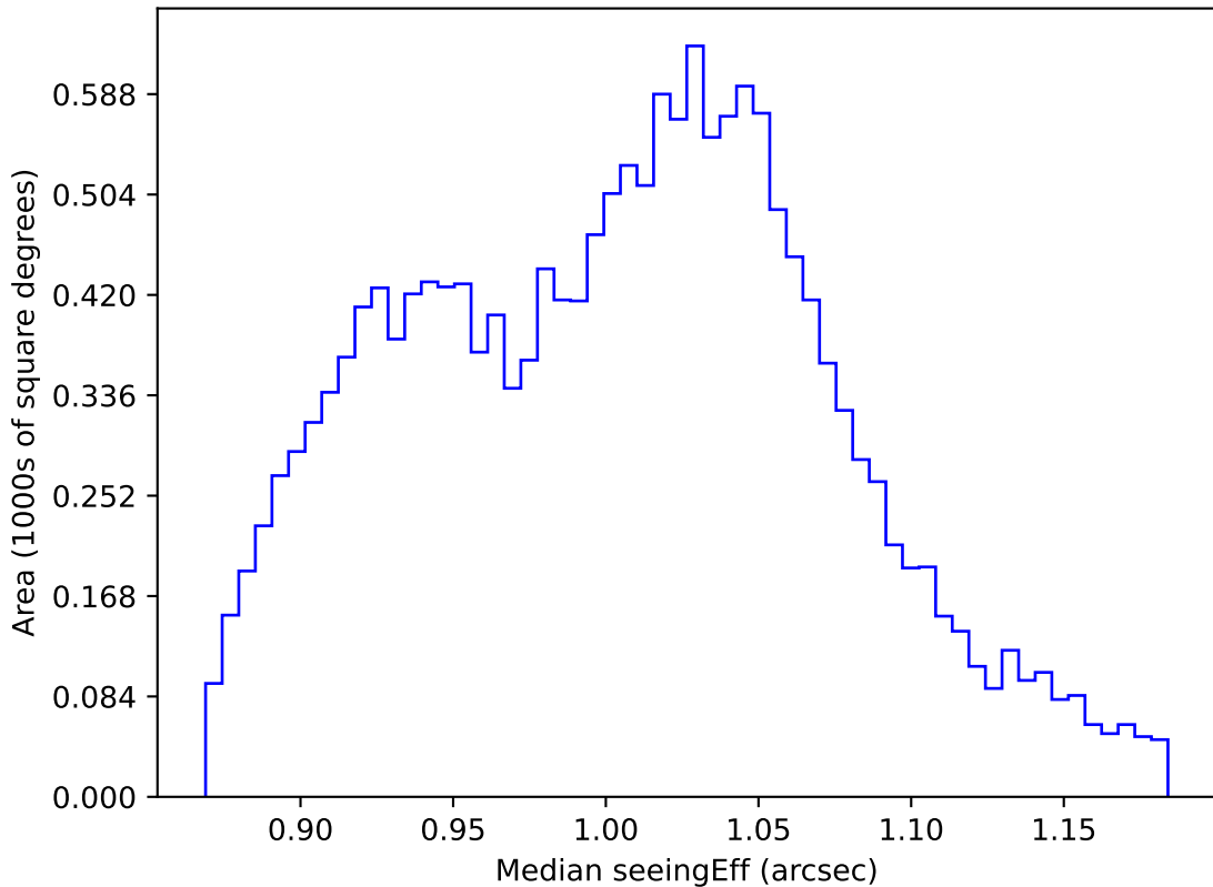
too_ignore_5_1v3.4_10yrs WFD z band: Median seeingEff
