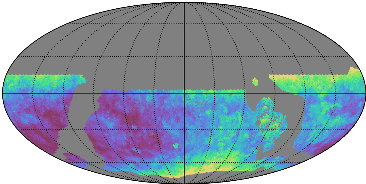
too_ignore_5_1v3.4_10yrs WFD y band: Median seeingEff
