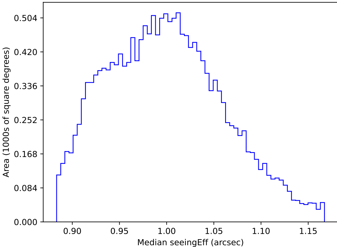
too_ignore_5_1v3.4_10yrs WFD y band: Median seeingEff
