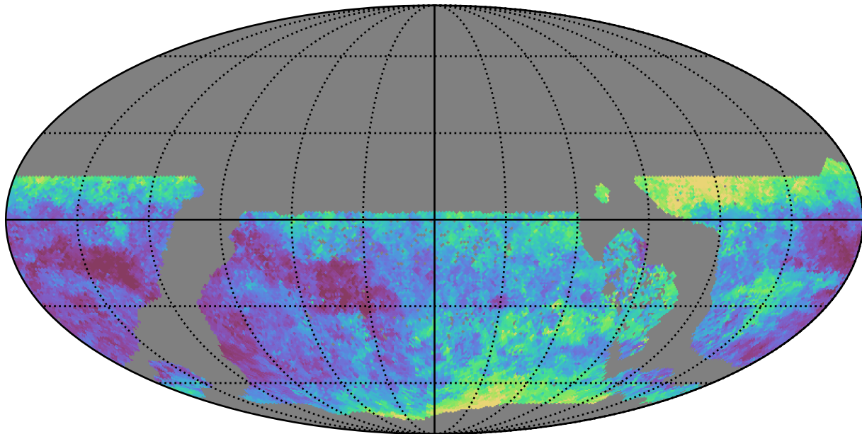
too_ignore_5_1v3.4_10yrs WFD u band: Median seeingEff
