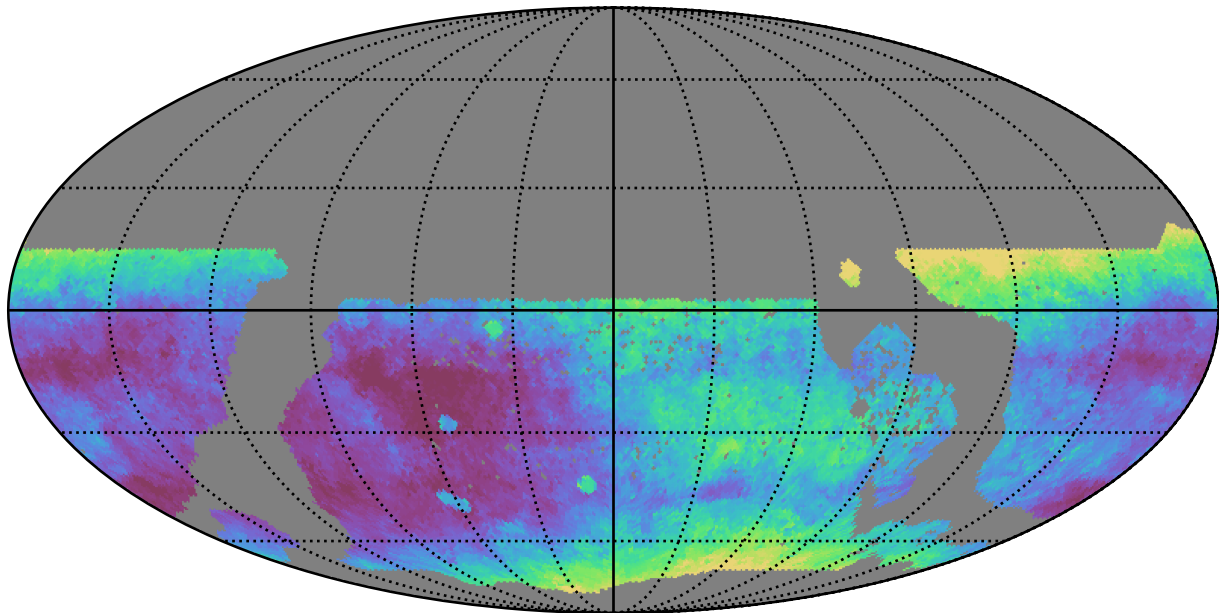
too_ignore_5_1v3.4_10yrs WFD r band: Median seeingEff
