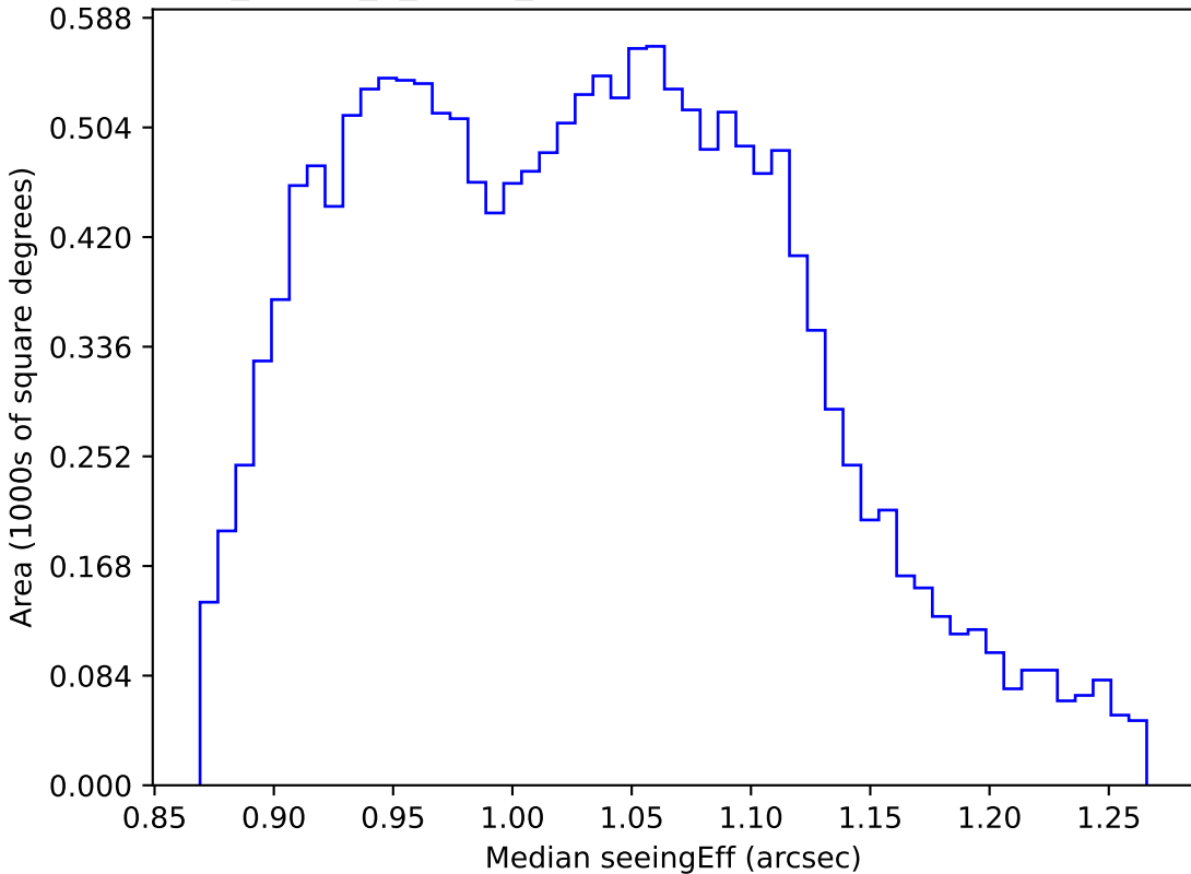
too_ignore_5_1v3.4_10yrs WFD r band: Median seeingEff
