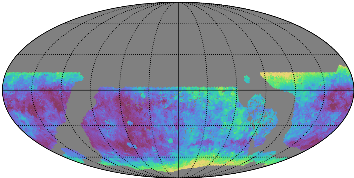
too_ignore_5_1v3.4_10yrs WFD g band: Median seeingEff
