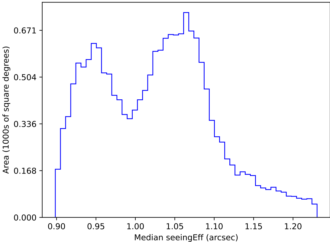
too_ignore_5_1v3.4_10yrs WFD all bands: Median seeingEff
