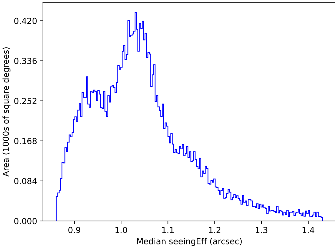
too_ignore_5_1v3.4_10yrs All sky z band: Median seeingEff
