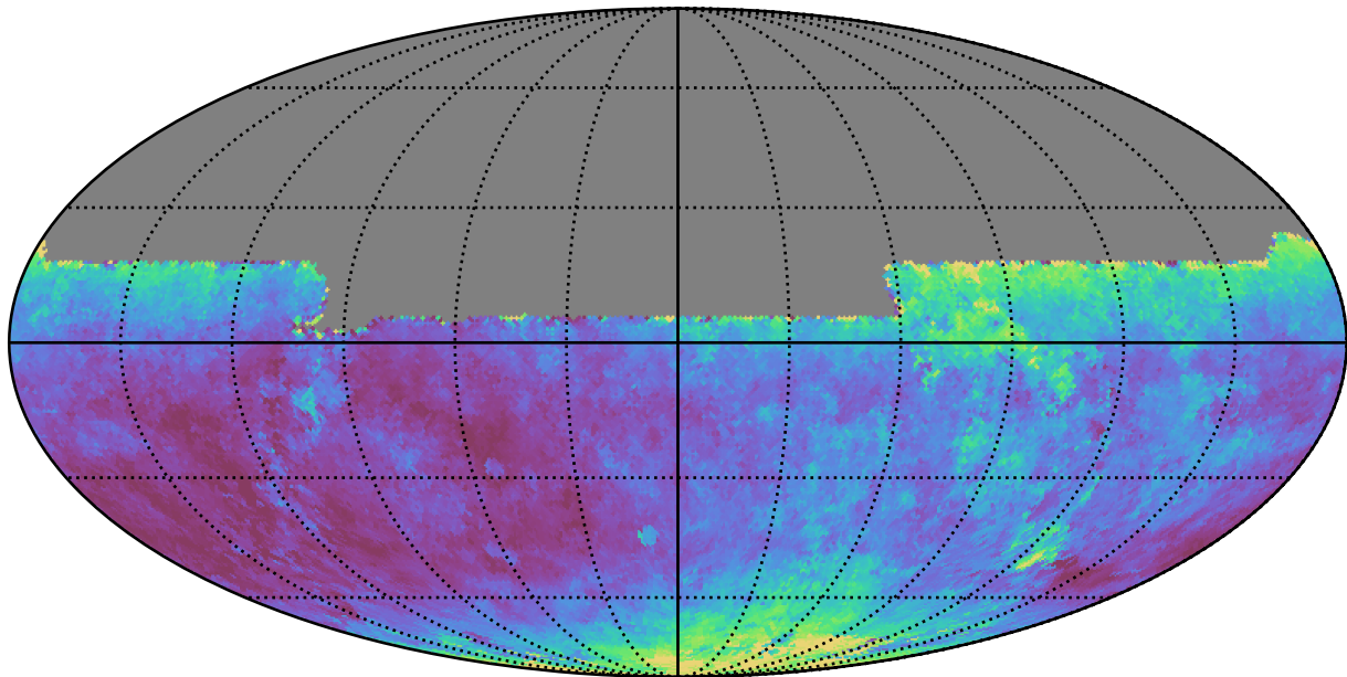
too_ignore_5_1v3.4_10yrs All sky y band: Median seeingEff
