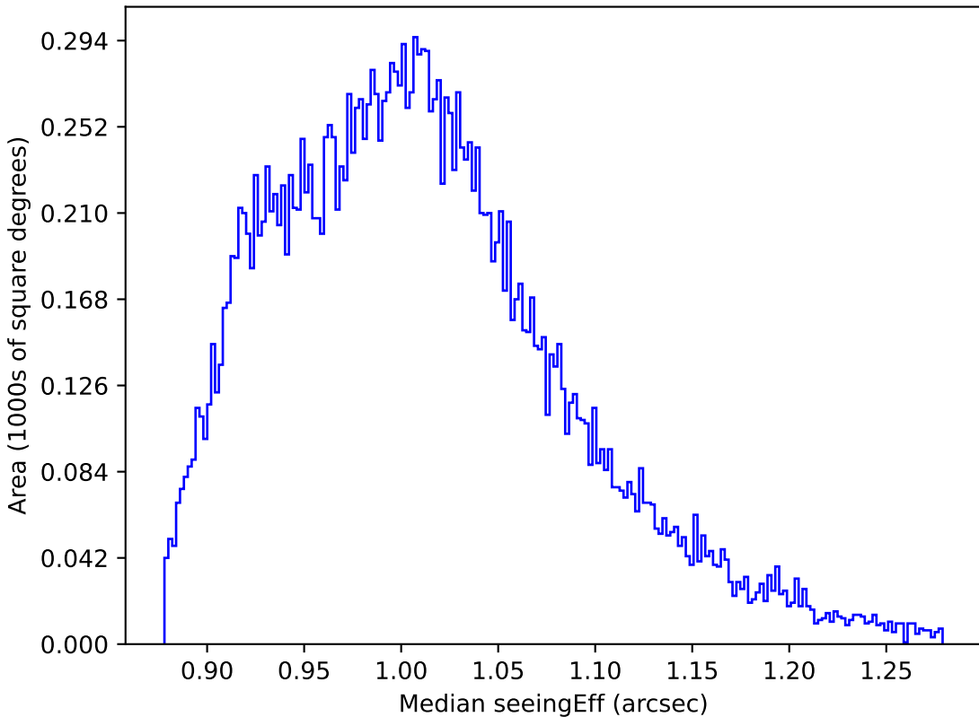
too_ignore_5_1v3.4_10yrs All sky y band: Median seeingEff
