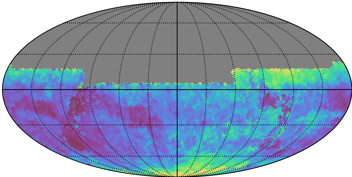
too_ignore_5_1v3.4_10yrs All sky u band: Median seeingEff
