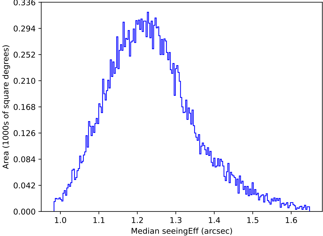
too_ignore_5_1v3.4_10yrs All sky u band: Median seeingEff
