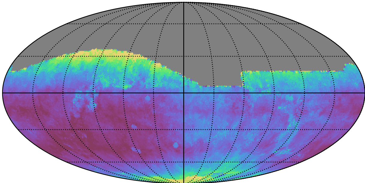
too_ignore_5_1v3.4_10yrs All sky i band: Median seeingEff
