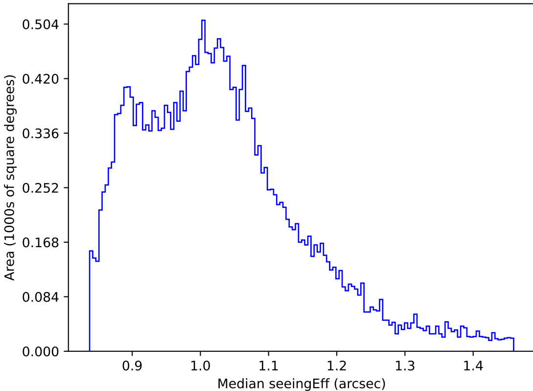
too_ignore_5_1v3.4_10yrs All sky i band: Median seeingEff
